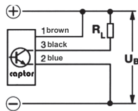
NPN- transistor output
