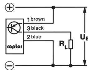
PNP- transistor output
