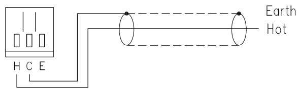
Connection Diagram
