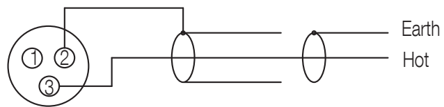
Connection Diagram
