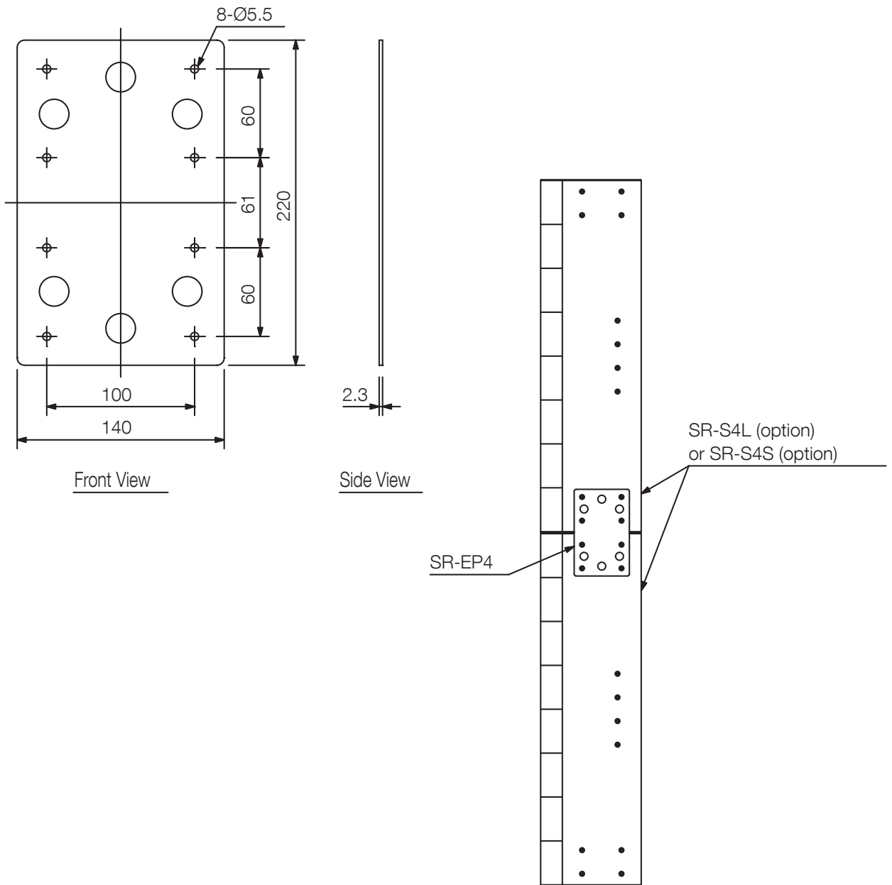
Mounting example (scale: 1/15)
