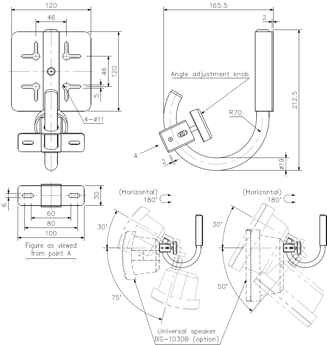
Mounting example
