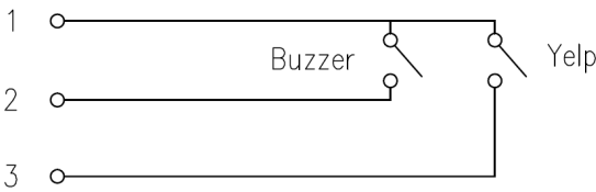
Connection Diagram
