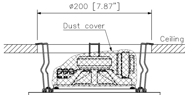
Mounting Diagram
