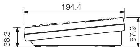
Figure of the desktop installation (scale: 1/5)
