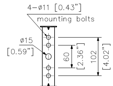
Dimension for mounting hole (U bracket (accessory))
