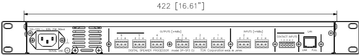
Rear View
