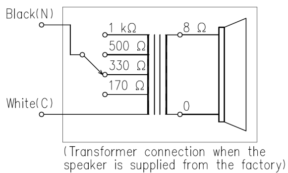
Wiring Diagram
