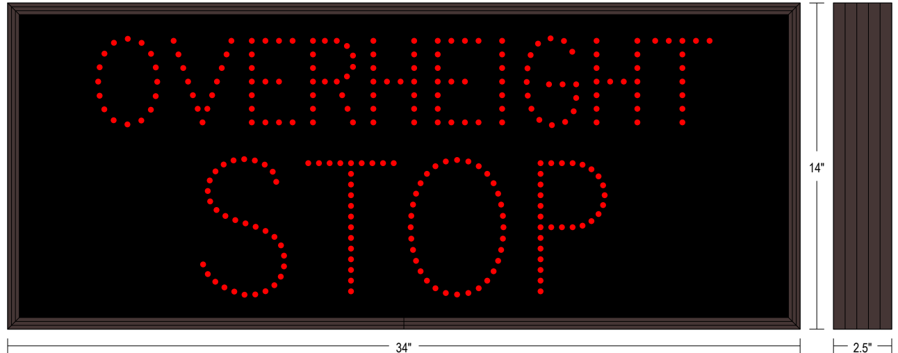
Frame Detail
