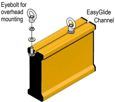
I-Bar Detail
