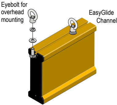
I-Bar Detail
