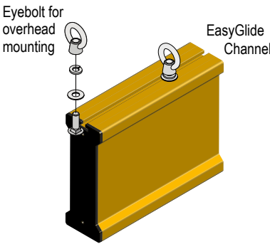
I-Bar Detail
