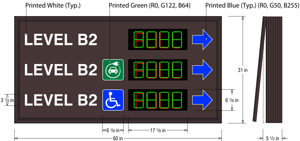
Frame Detail
