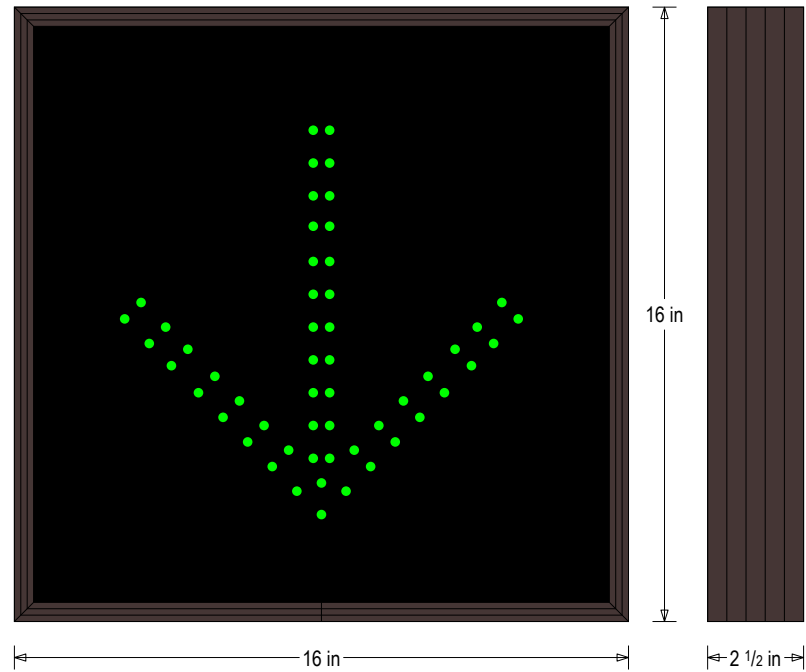
Frame Detail
