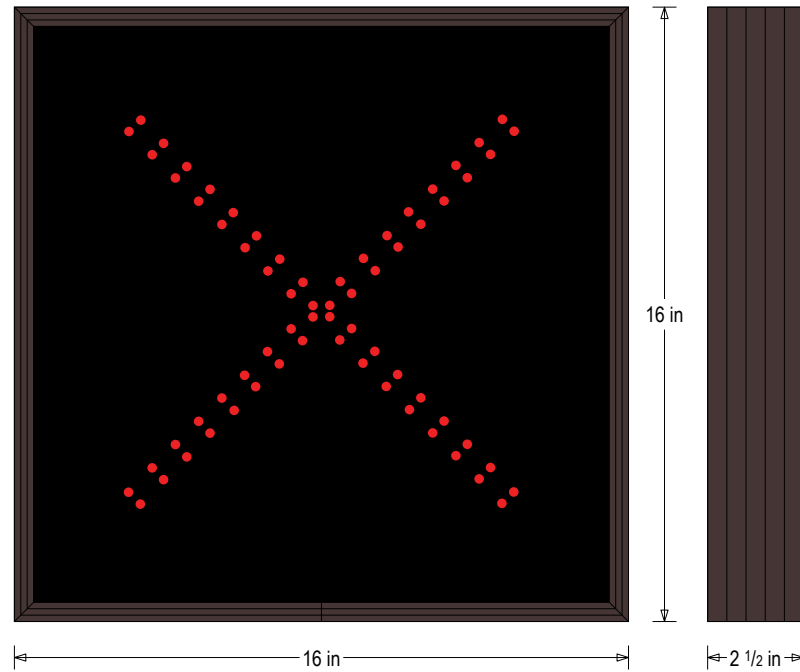
Frame Detail
