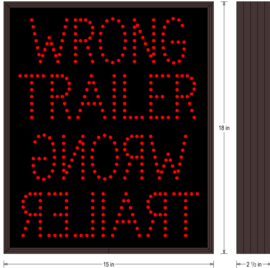
Frame Detail
