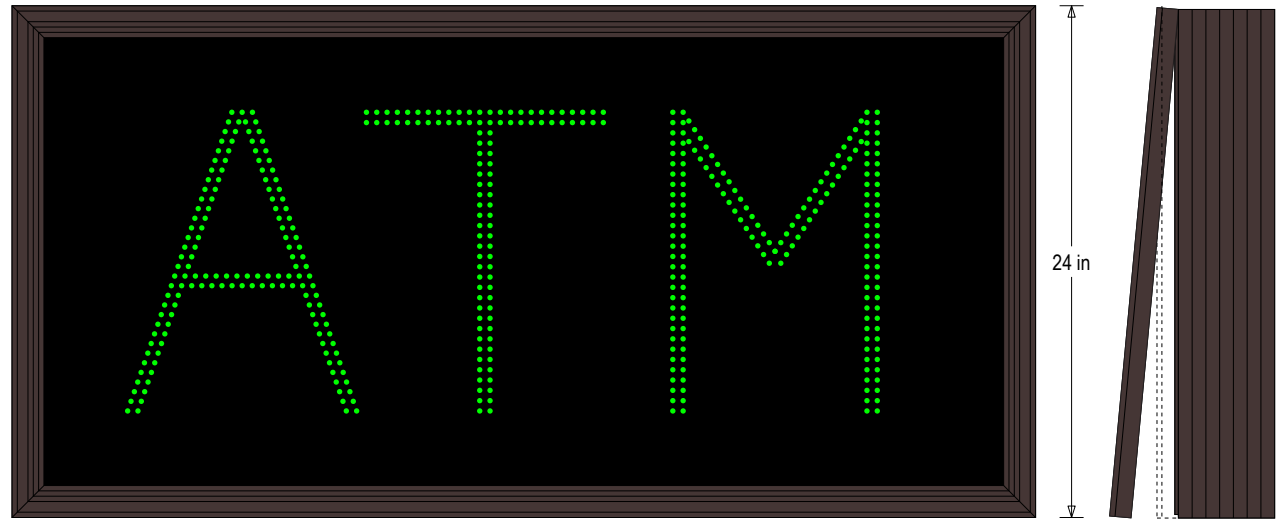
Frame Detail
