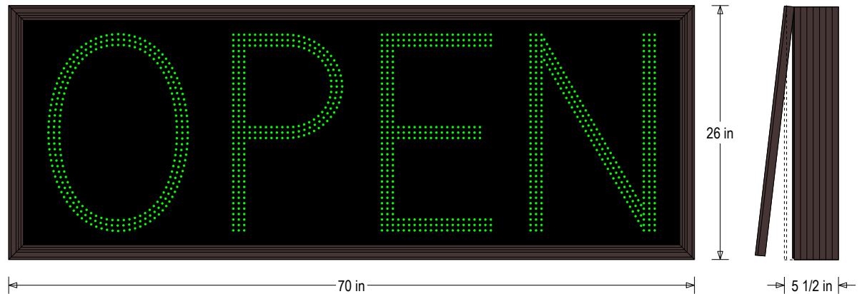
Frame Detail
