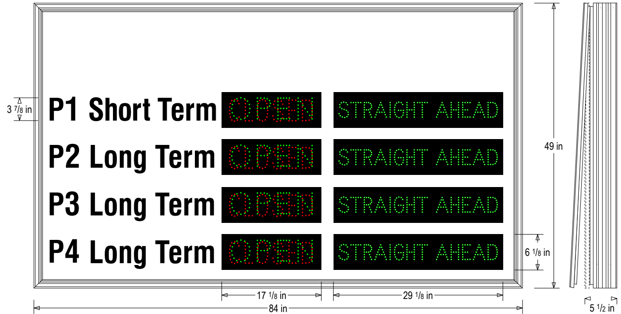
Frame Detail
