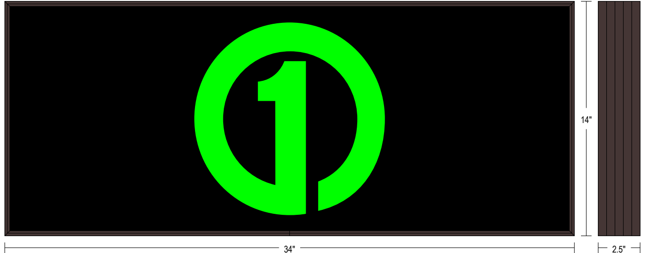
Frame Detail
