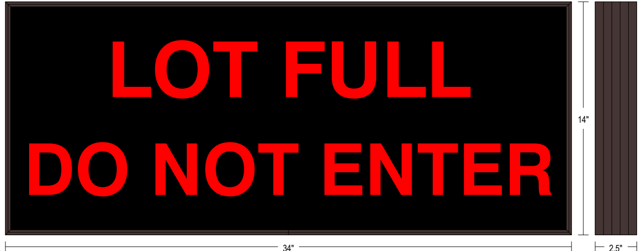
Frame Detail
