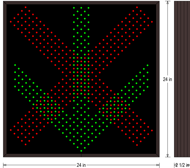
Frame Detail
