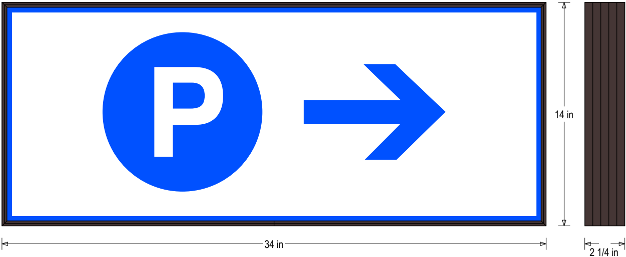
Frame Detail
