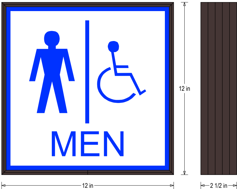
Frame Detail
