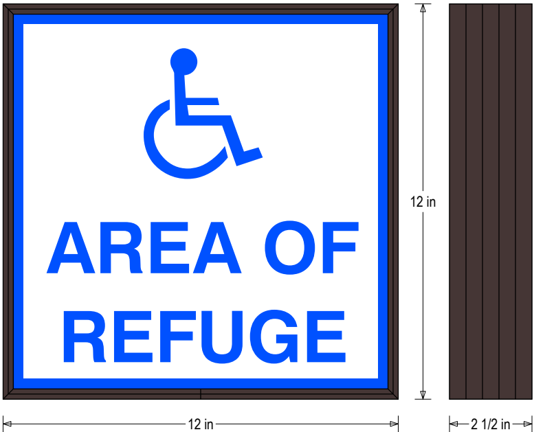
Frame Detail
