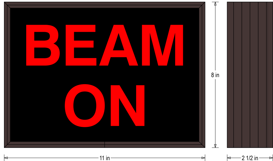
Frame Detail
