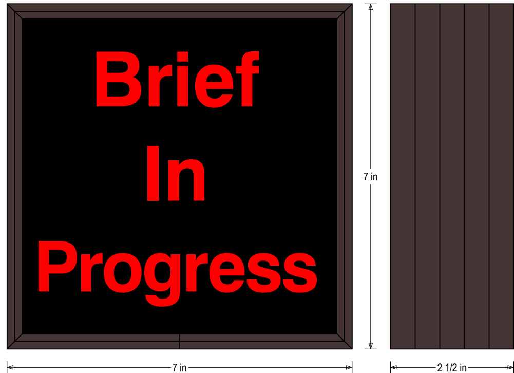
Frame Detail
