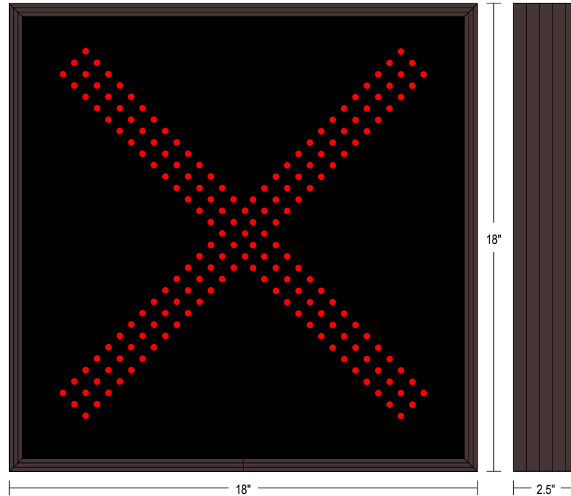
Frame Detail
