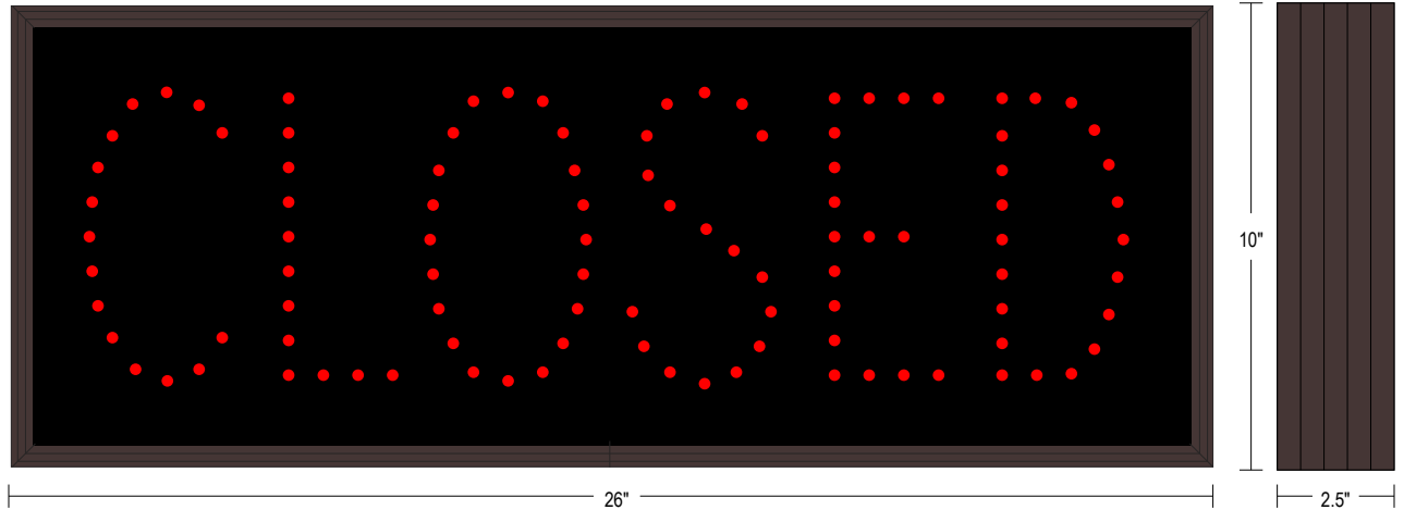
Frame Detail
