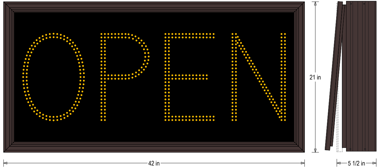
Frame Detail
