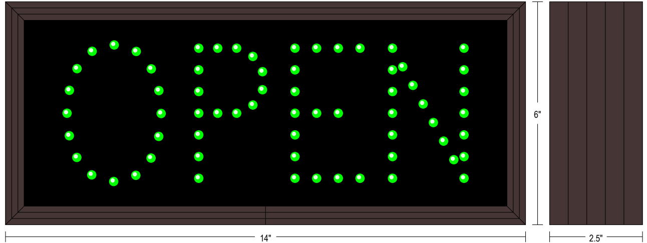
Frame Detail
