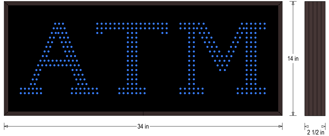
Frame Detail
