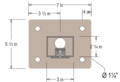
Baseplate Detail
