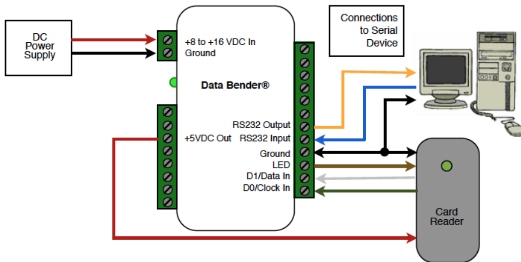
DB-9 Connections Direct to PC Com Port
