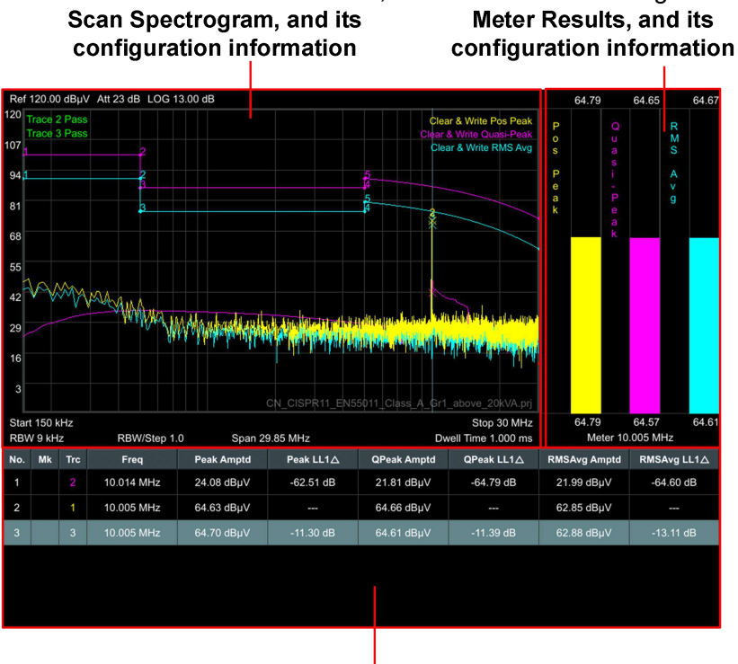
Figure 6-1 EMI measurement interface
