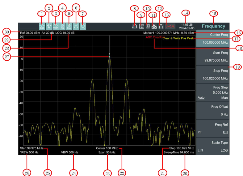
Figure 4- 7 User interface
