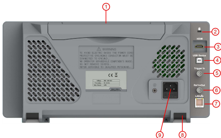
Figure 4-6 Rear Panel
