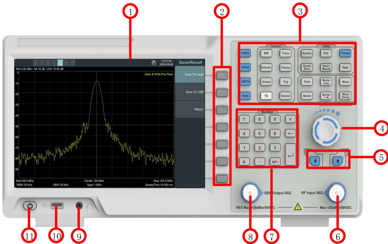
Figure 4- 1 Front panel
