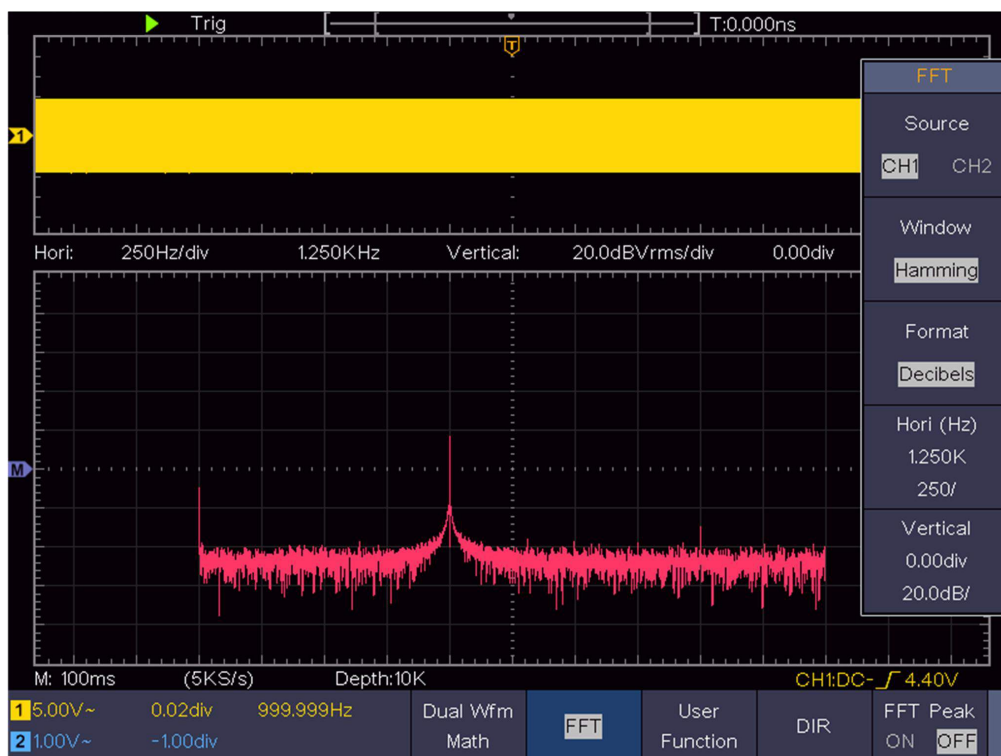
Figure 4- 1 Hamming window
