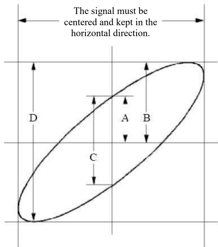
Figure 9-6 Lissajous Graph
