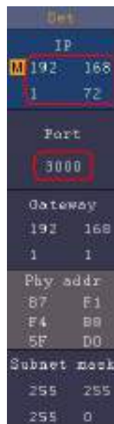
Figure 7-4 Set the network parameters of the oscilloscope
