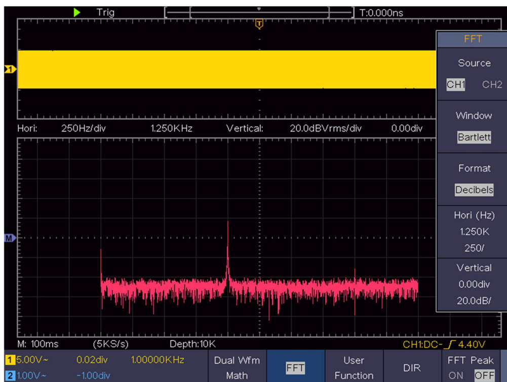
Figure 4- 6 Bartlett window
