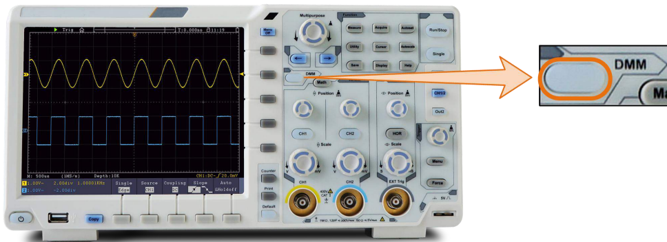
Figure 6-2 Multimeter Button
