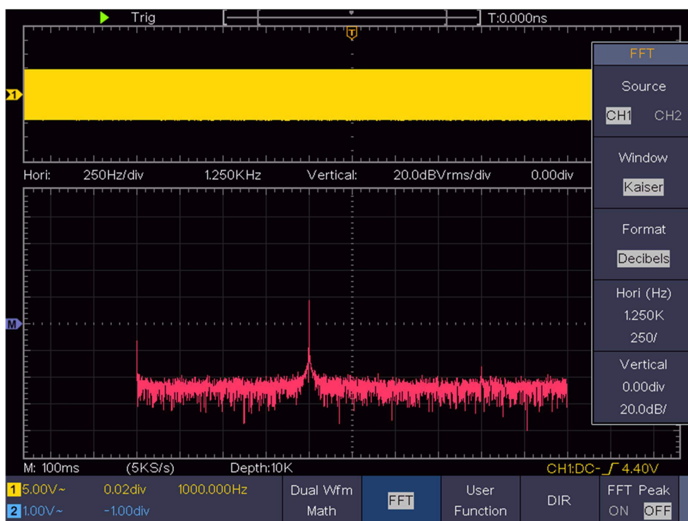
Figure 4- 5 Kaiser window
