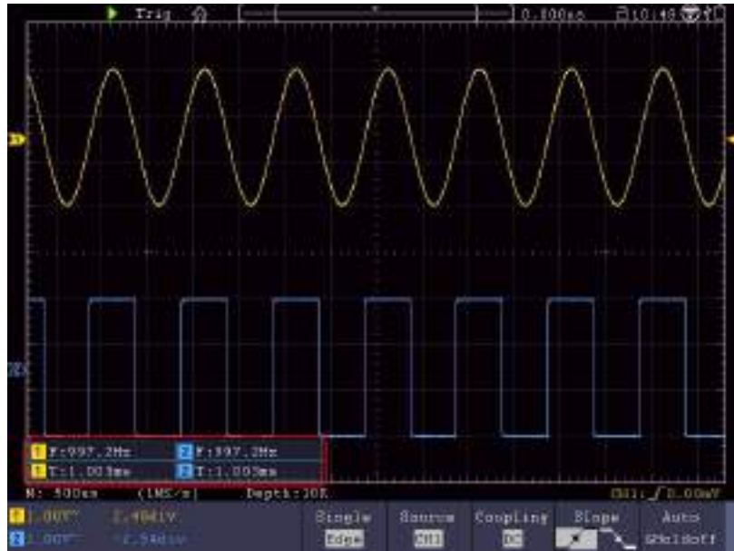
Figure 4-20 Automatic measurement
