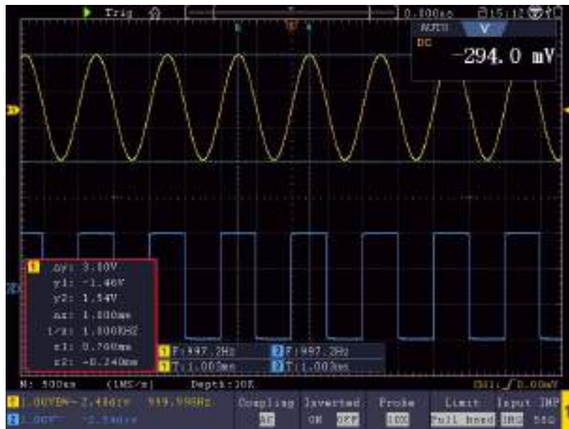
Figure 4-23 Time&amp;Voltage Cursor Measurement
