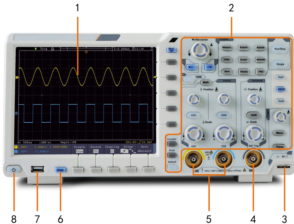
Figure 3- 1 Front panel
