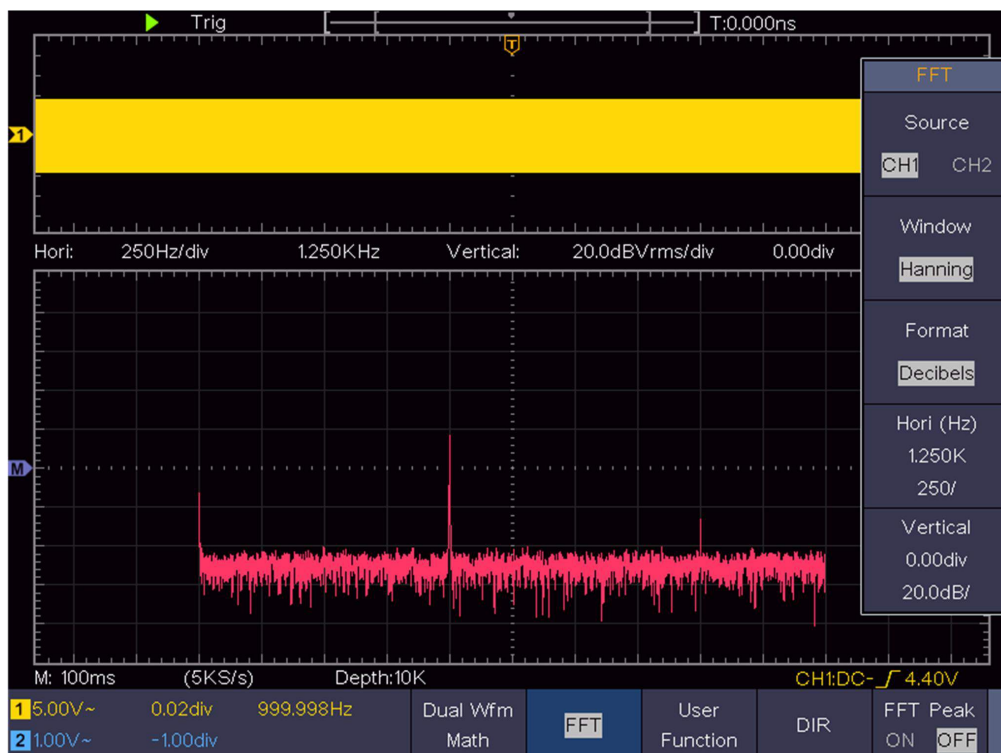
Figure 4- 4 Hanning window
