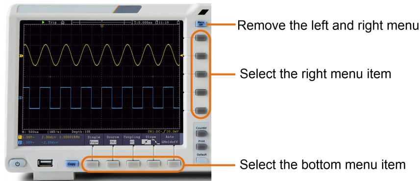
Figure 3-2 Menu Buttons
