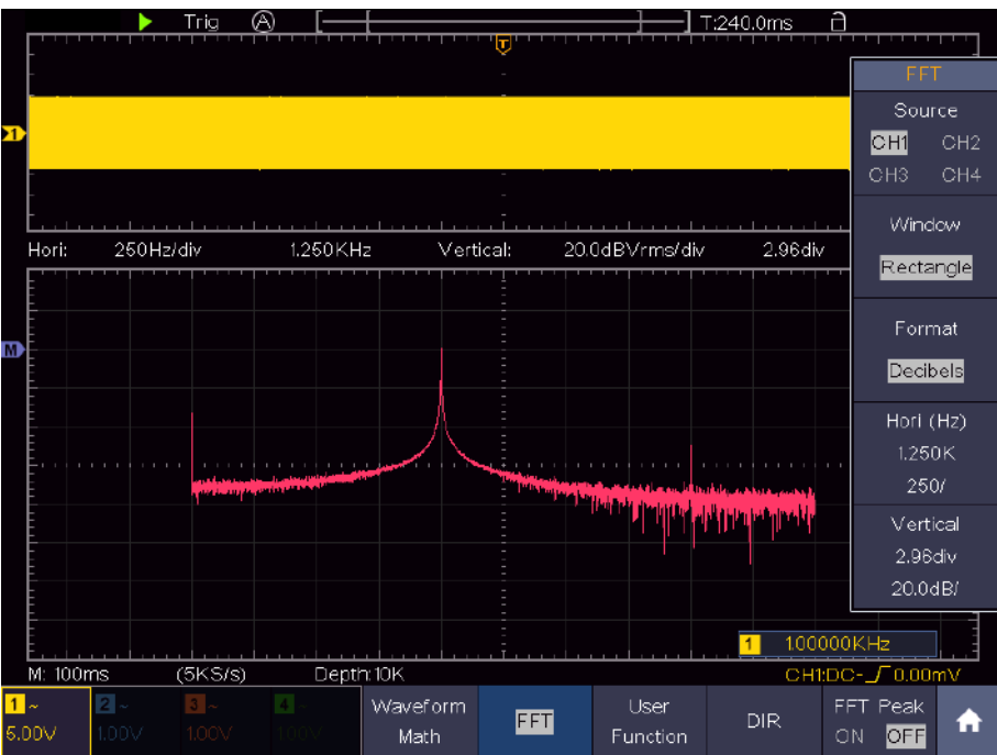
Figure 4-2 Rectangle window
