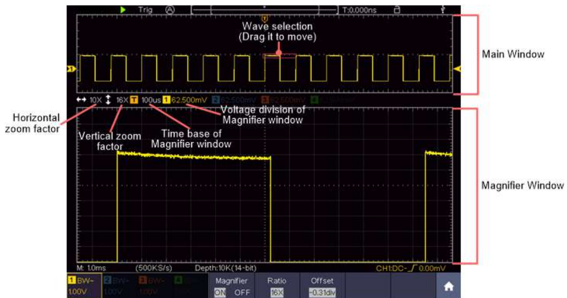
Figure 4-9 Magnifier Mode
