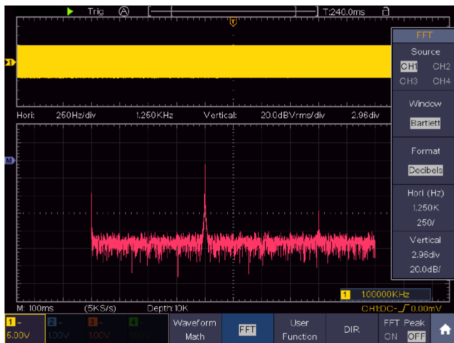
Figure 4-6 Bartlett window
