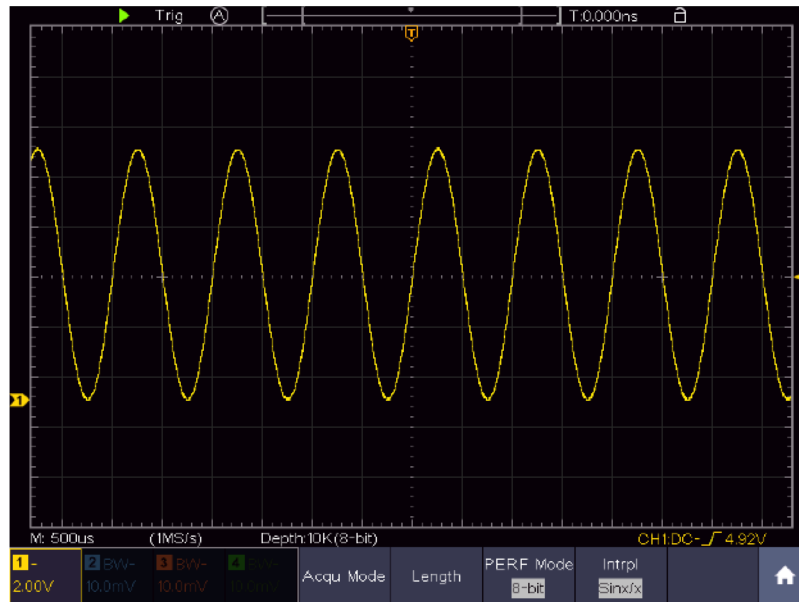
Figure 4-10 Sine(x)/x interpolation
