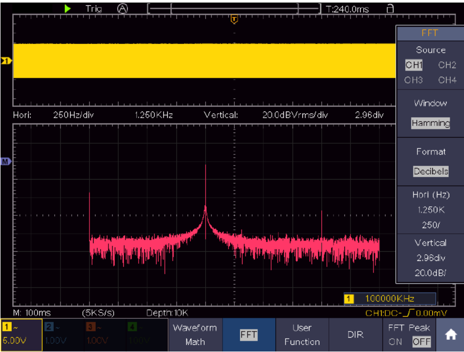
Figure 4-1 Hamming window
