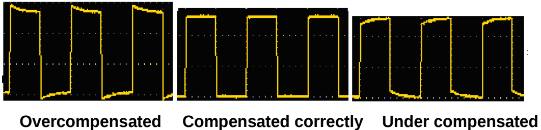
Figure 3-6 Displayed Waveforms of the Probe Compensation
