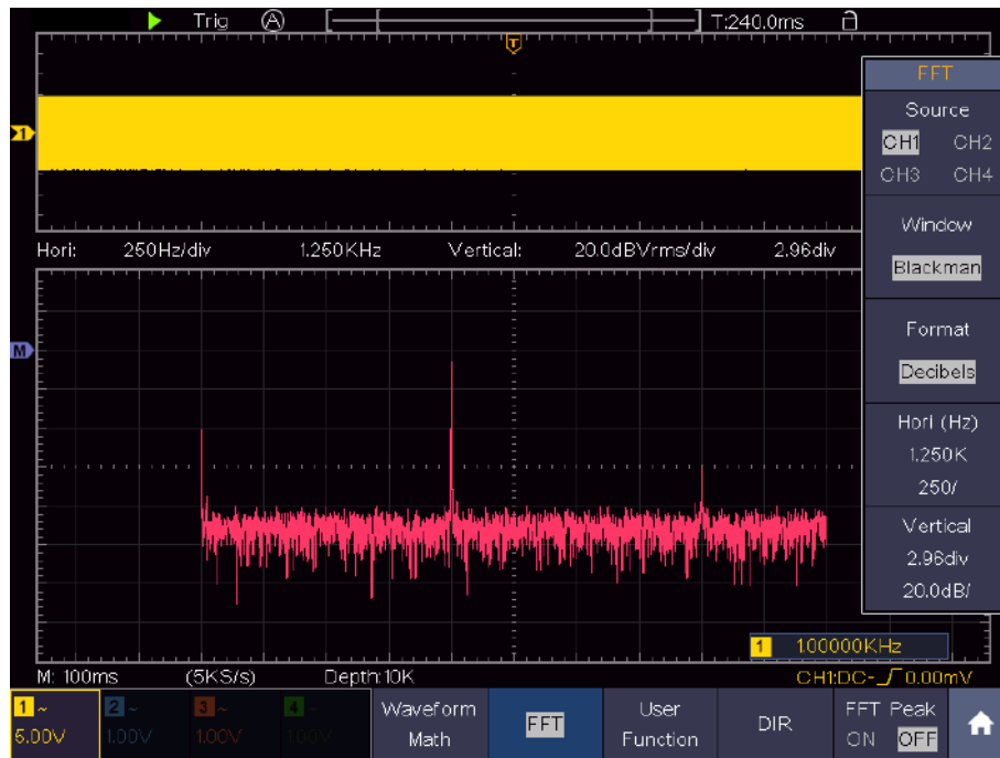
Figure 4-3 Blackman window
