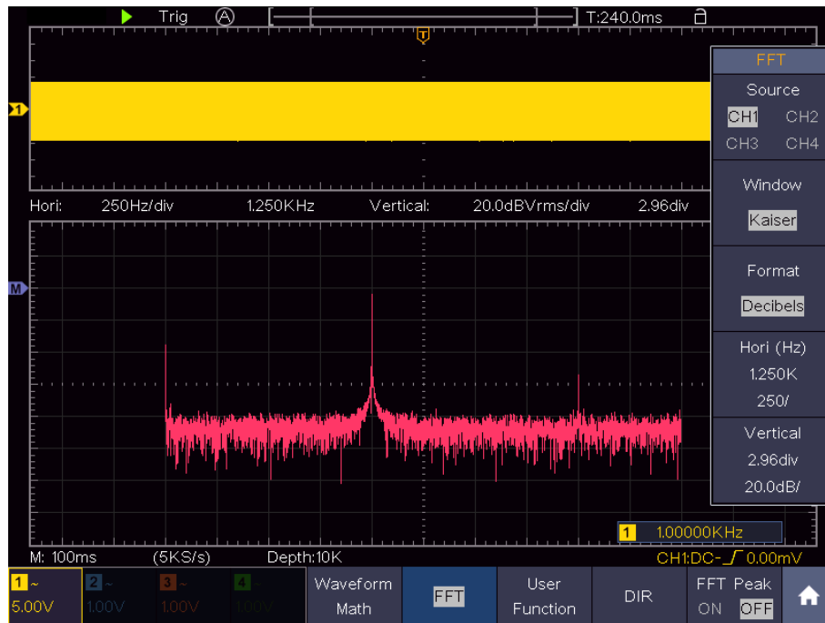
Figure 4-5 Kaiser window
