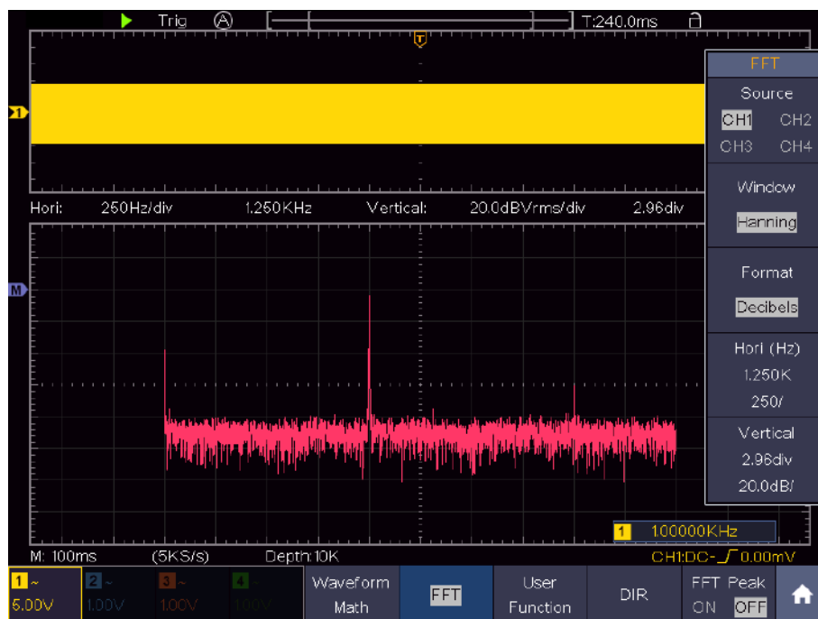
Figure 4-4 Hanning window
