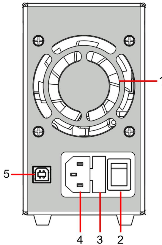
Figure 3-2 Rear Panel Overview(Without L model)
