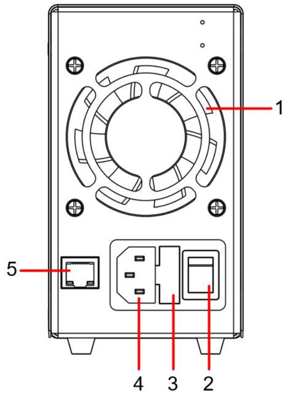
Figure 3-3 Rear Panel Overview (With L model)
