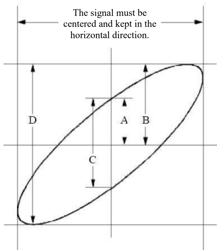
Figure 6-6 Lissajous Graph
