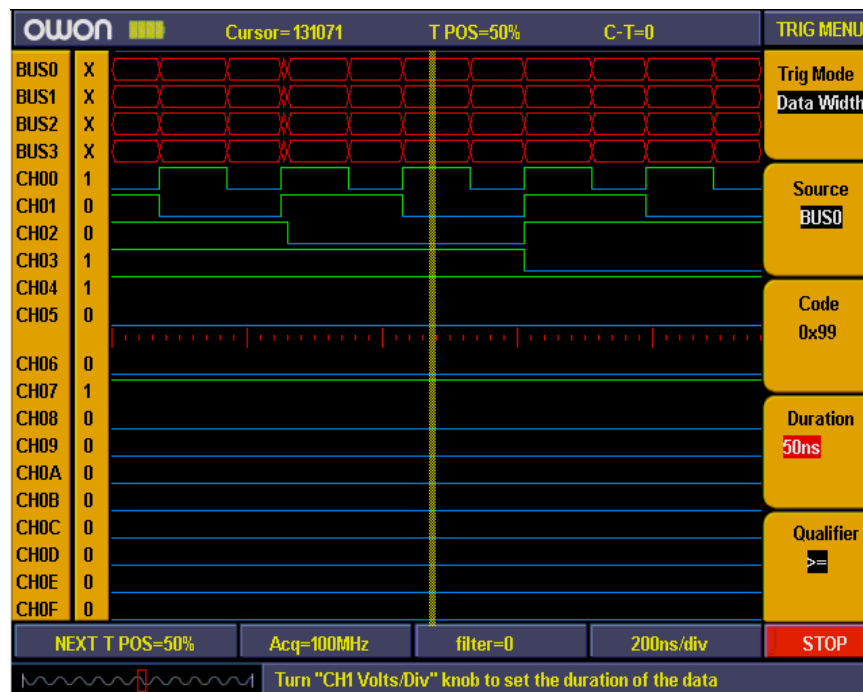
Fig.5-65: Data width trigger
