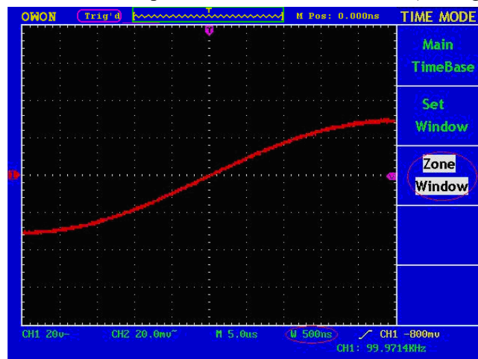
Fig. 5-18 Zone Window
