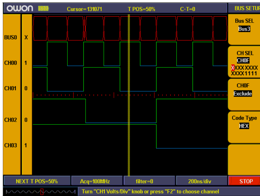
Fig.5-71: Bus setting
