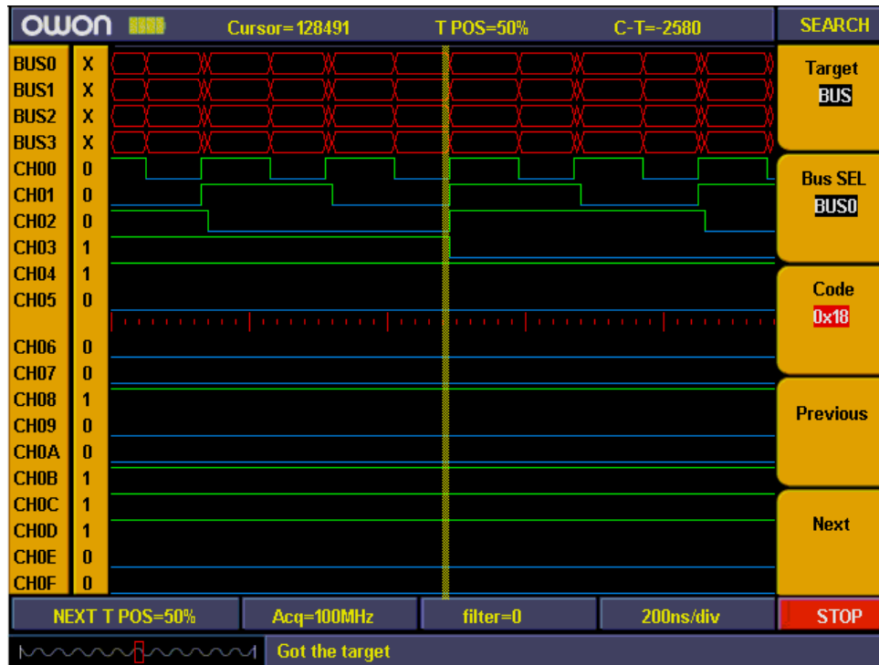
Fig.5-76.: Search Bus
