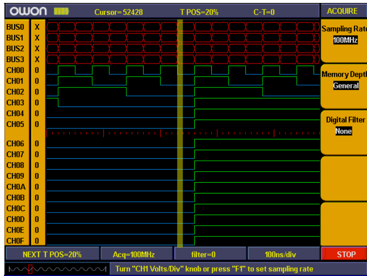
Fig. 5-53: Sampling setting
