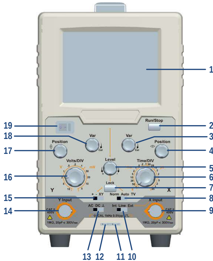
Figure 3-1 Front panel
