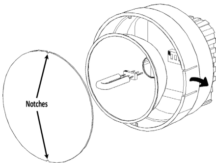
Figure 4 Lamp Replacement
