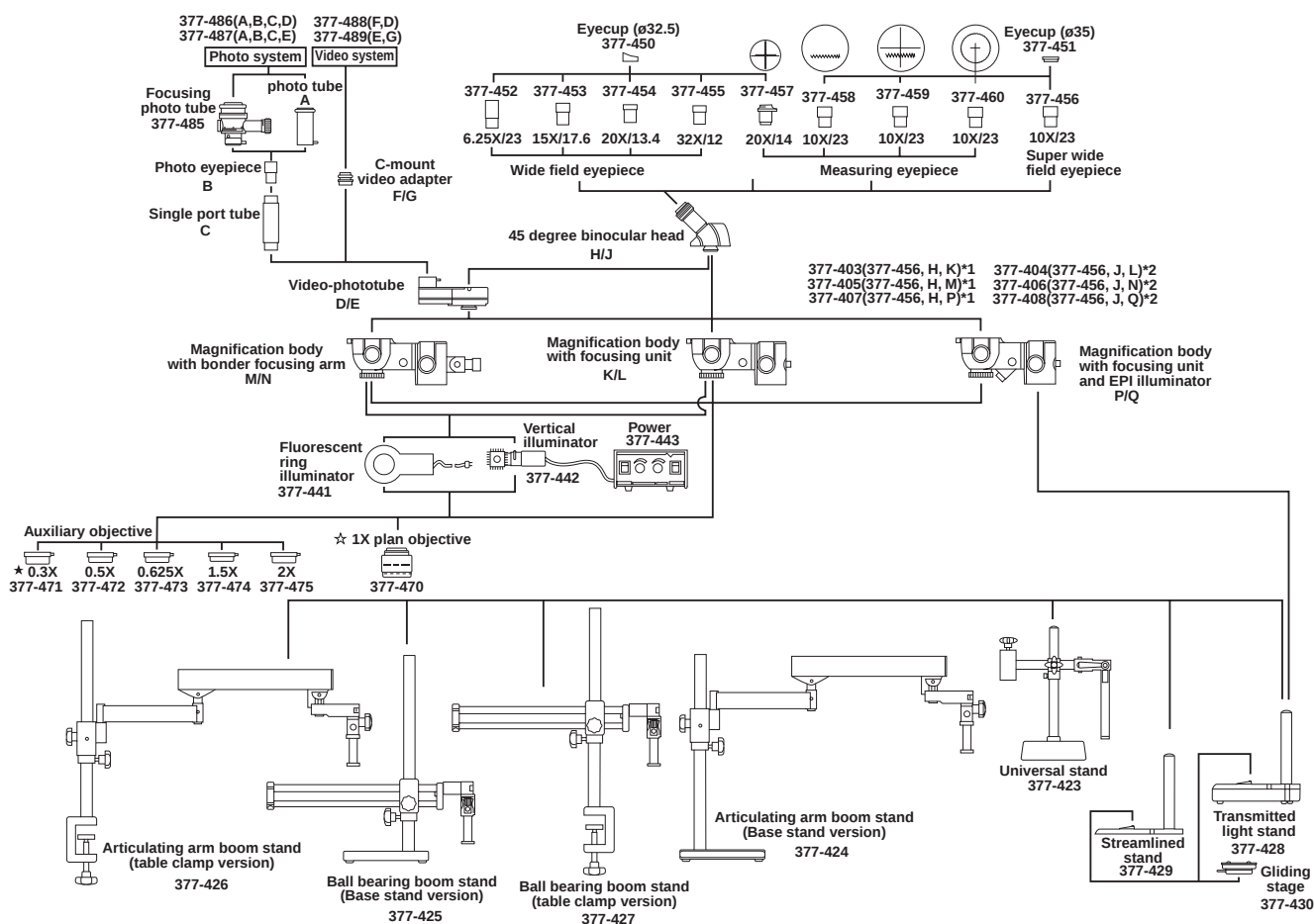
377-990A/377-991A SYSTEM DIAGRAM
