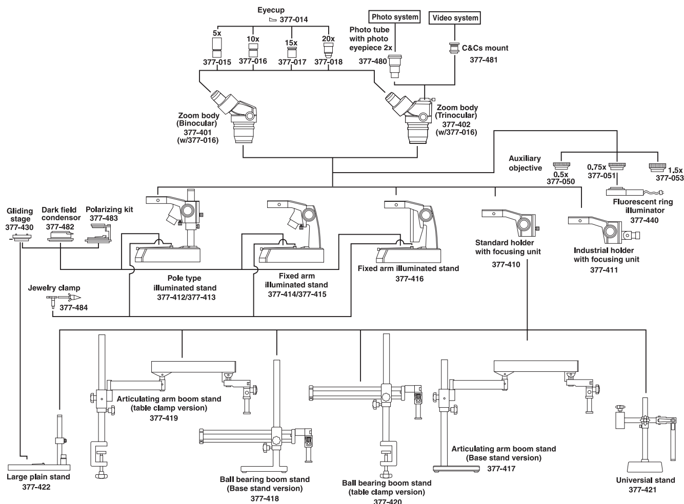
377-972A/377-974A SYSTEM DIAGRAM
