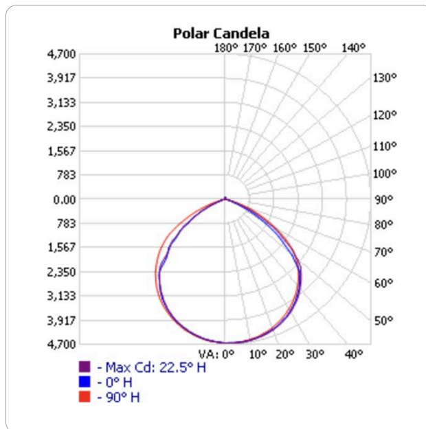
FLLS-40T80W-3CCT-DV2-PC-BZKM
