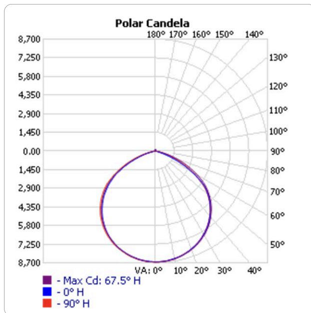
FLLS-100T150W-3CCT-DV2-PC-BZAM
