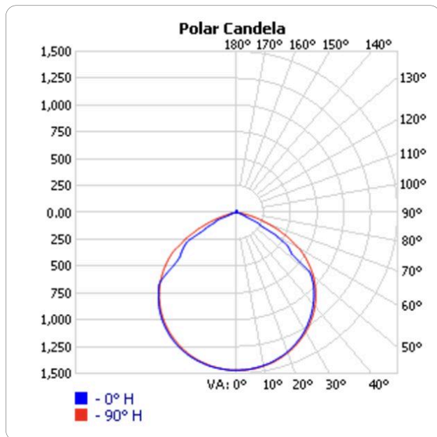
FLLS-15T35W-3CCT-DV2-PC-BZKM
