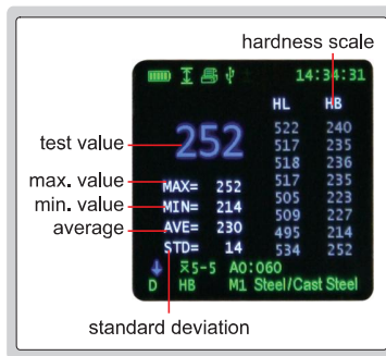
statistic display
