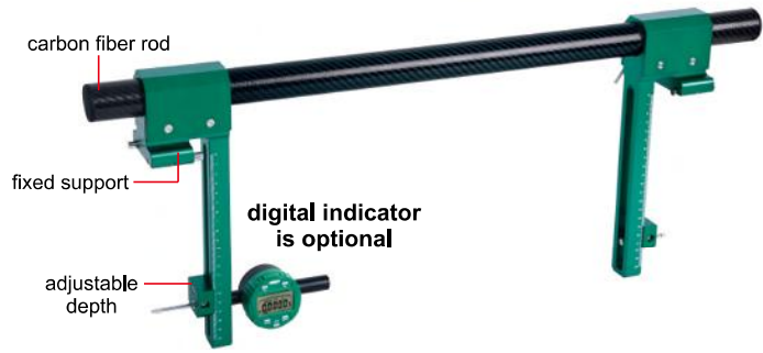
measure inside diameter, minimum diameter is 9"
